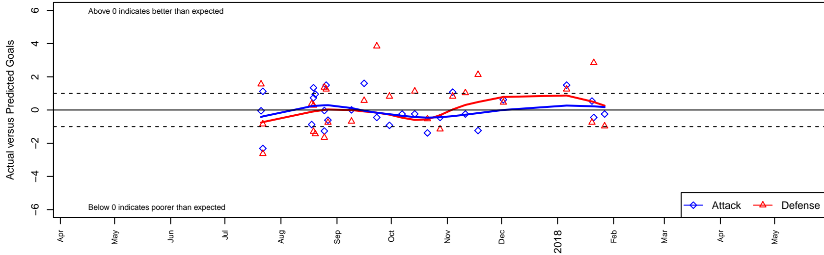
Norpoint FC B05 Dots are actual minus expected GF (blue circles) and GA (red triangles). Blue line is smoothed change in attack strength. Red is smoothed change in defense strength.
